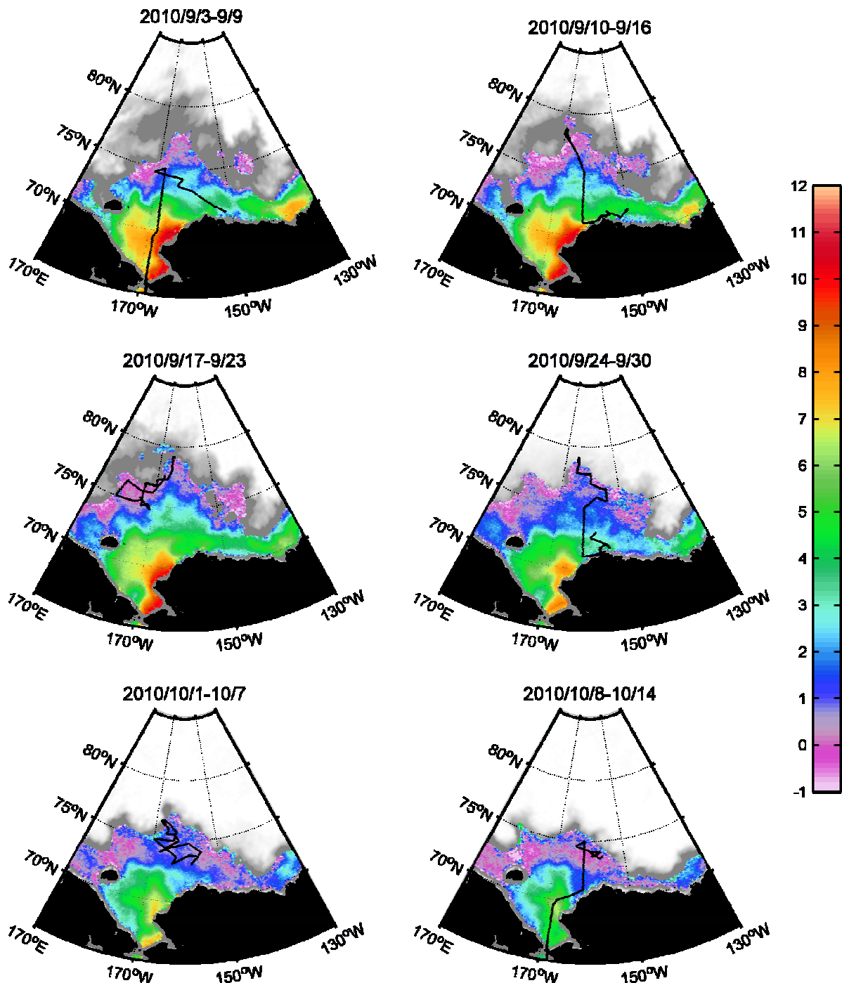
Time series of sea-ice concentration and sea surface temperature, deduced from Advanced Microwave Scanning Radiometer for Earth Observing System (AMSRE) data. The cruise tracks are superimposed.
