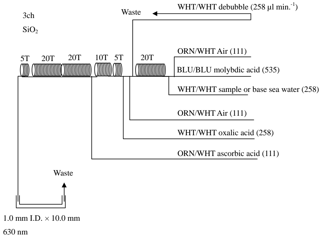
Figure4.2-4 SiO 2 (3ch.) Flow diagram.
