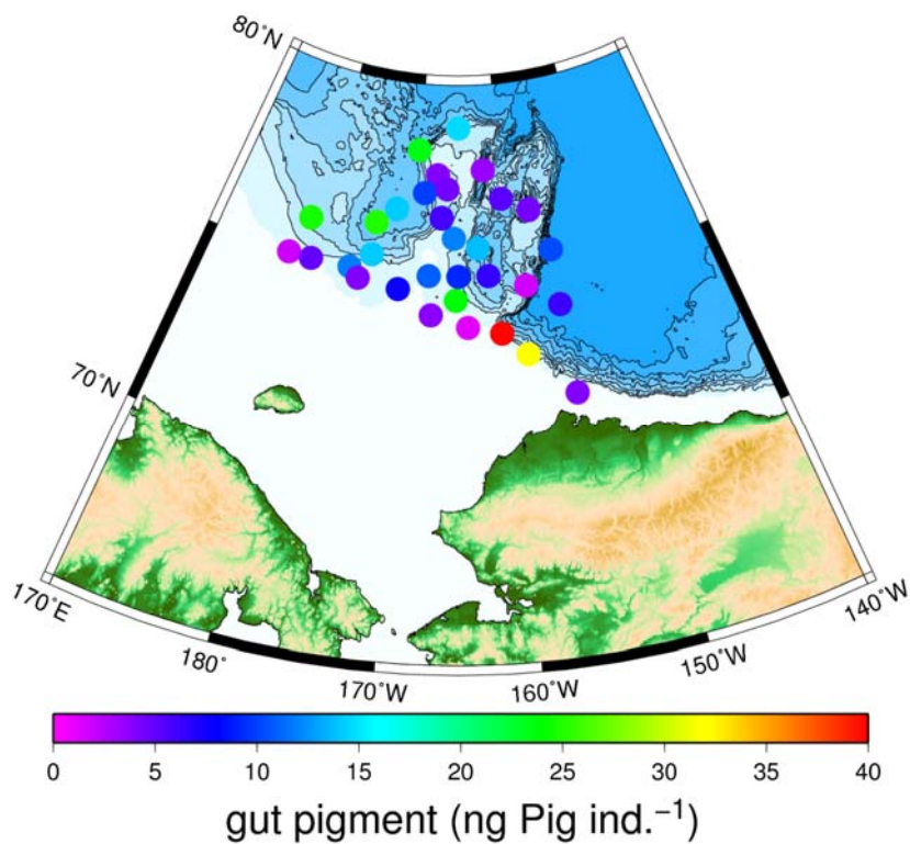
Fig. 4.14-5. Geographical distribution of gut pigment of Metridia longa C6F.
