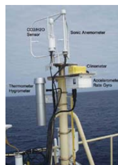
Fig. 2.7-1. Turbulent flux measurement system on the top deck of the foremast.
