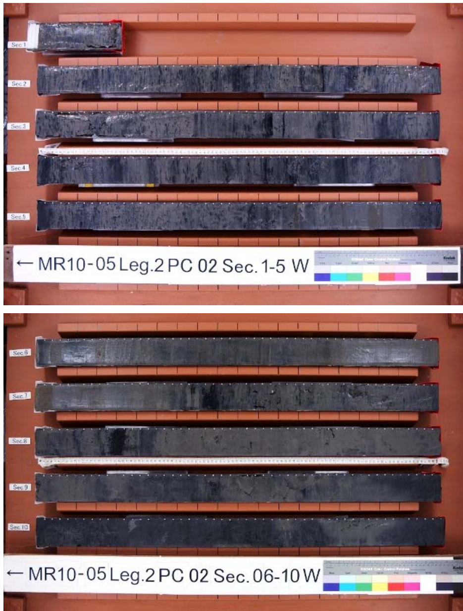
Figure 5.1-9. Photographs of W-half core PC02 sec.01 – 10.
