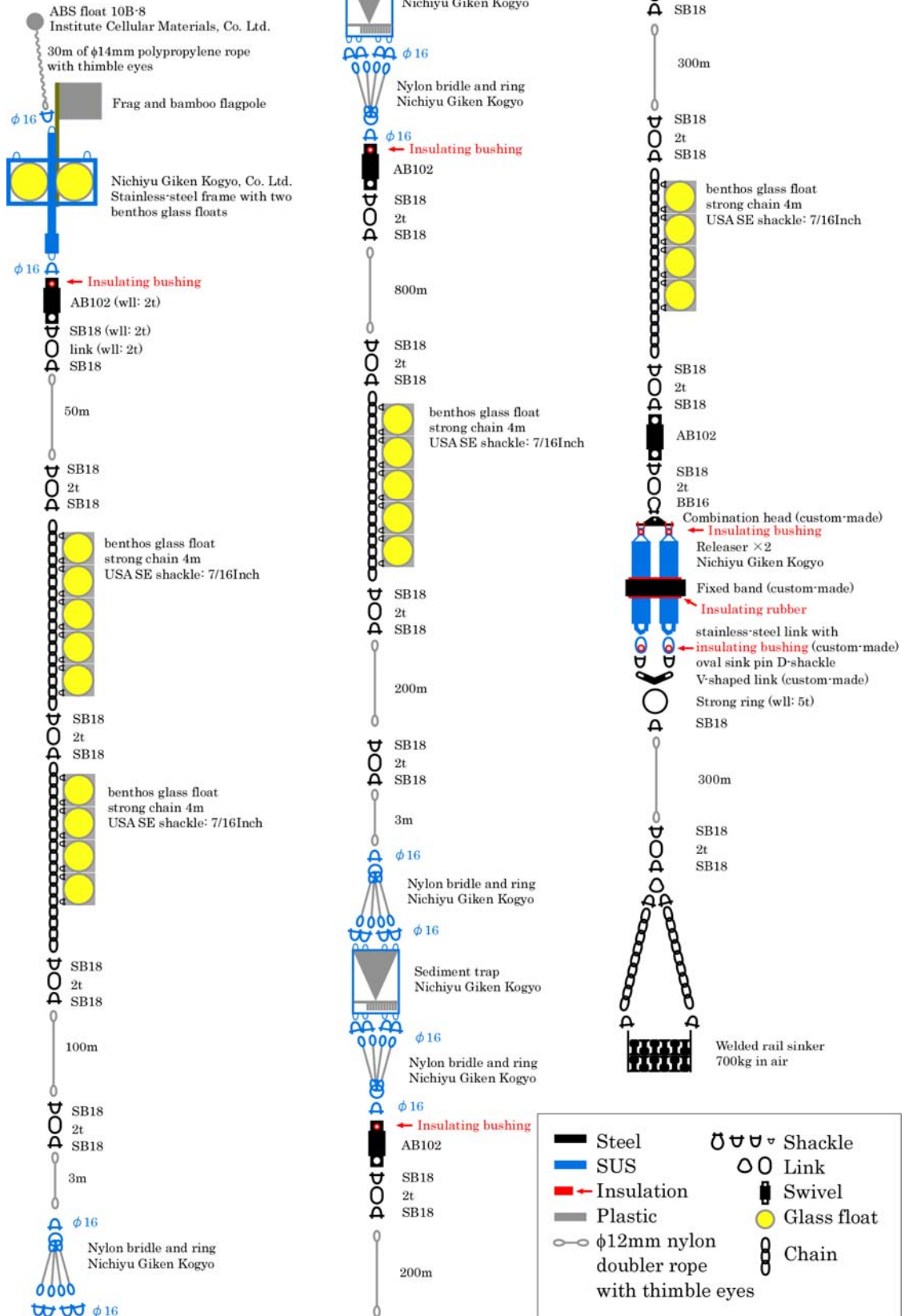
Figure 4.15-3. The layout of sediment trap mooring at Station CAP10t.
