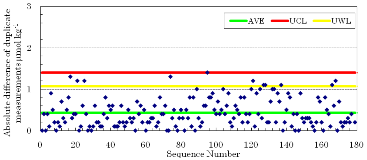
Fig. 4.6-2. Range control chart of the absolute differences of duplicate measurements carried out in the analysis of TA during this cruise. UCL and UWL represents the upper control limit ( \text{UCL}=\text{AVE}\times 3.267 ) and upper warning limit ( \text{UWL}=\text{AVE}\times 2.512 ), respectively.
