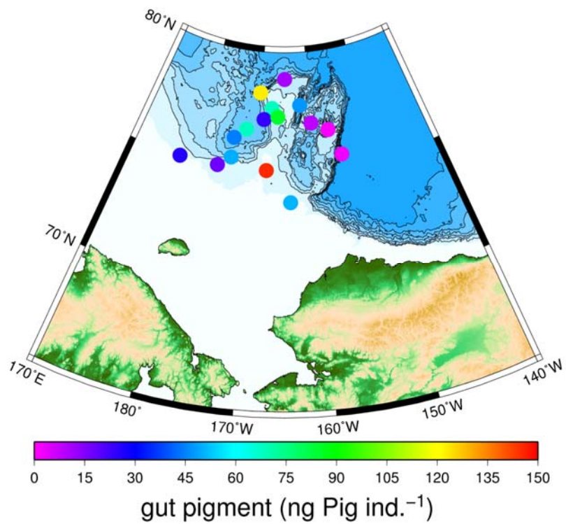
Fig. 4.14-4. Geographical distribution of gut pigment of Calanus hyperboreus C6F.
