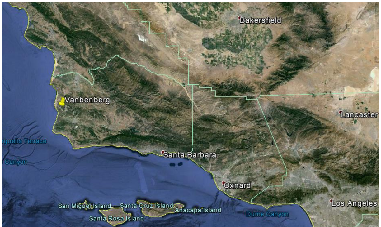
Figure 1. Location of the USAF Vandenberg AFB radiosonde release location.
