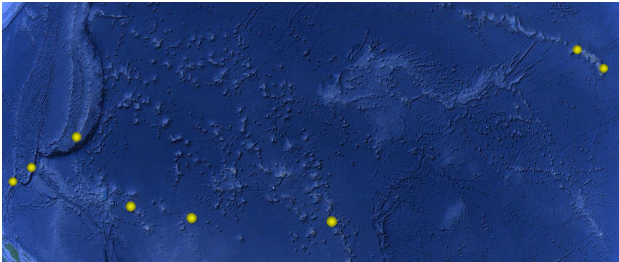
Figure 1. Locations of the 8 NWS release locations included in the CONTRAST data set.
