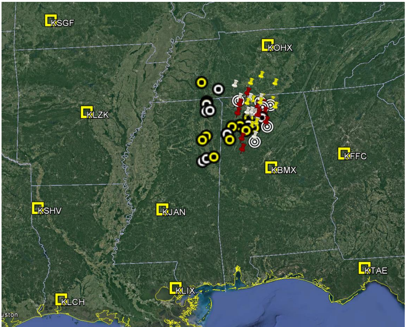
Figure 1. Locations of the soundings included in the VORTEX-SE 2016 composite data set. The NWS sites are the yellow squares. Purdue are the white pins, ULM the yellow pins, NOAA/ATDD the bullseyes, MSU iMet sondes the white circles, MSU WindSond sondes the yellow circles, and TTU the red pins.
