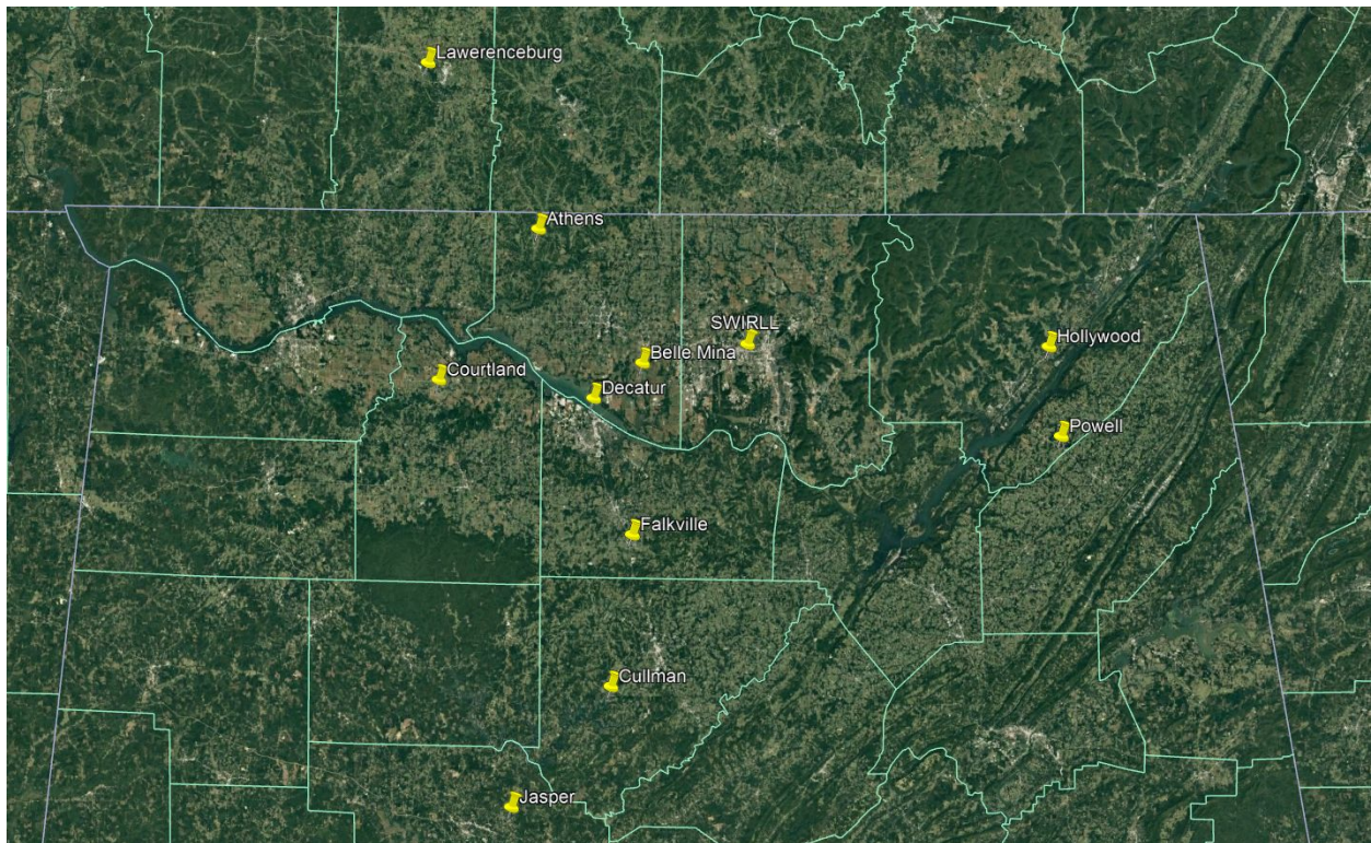
Figure 1. Locations of the UAH radiosonde sites.
