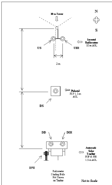
Figure 5. Plan View of SIRS Instrument Locations
