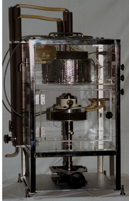
Figure 8. Photo of PIR BB Production 0809 Unit Blackbody Unit in Enclosure front view
