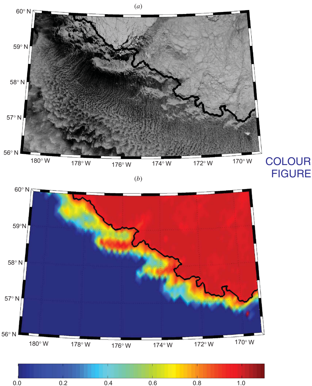
Figure 5. Comparison of erosion algorithm results for AMSR-E ice concentrations and high-resolution MODIS data on 10 March 2008. (a) MODIS image of calibrated radiance data (250 m resolution) and (b) AMSR-E image of sea ice concentration data. The black line in both panels is the final result after removing the marginal ice zone from pack ice using the erosion algorithm presented in this study.
