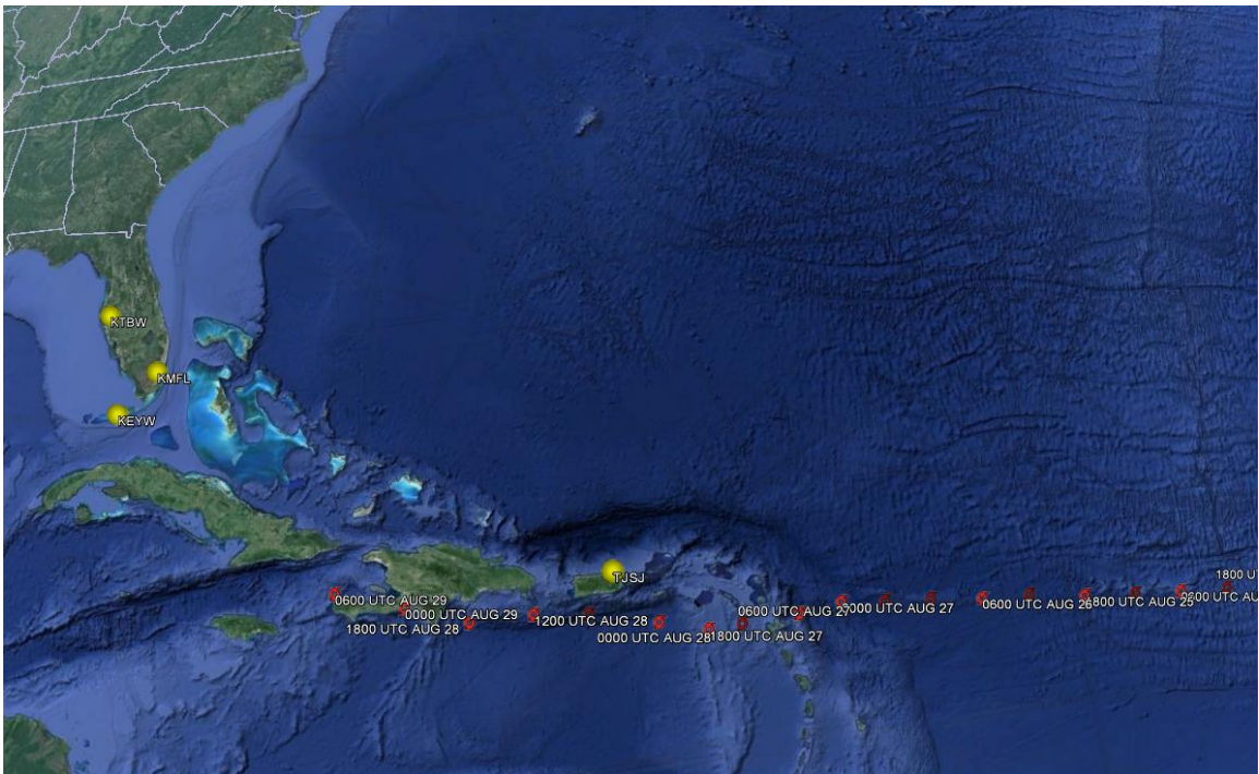
Figure 1. Tropical Storm Erika best track and NWS sounding locations.
