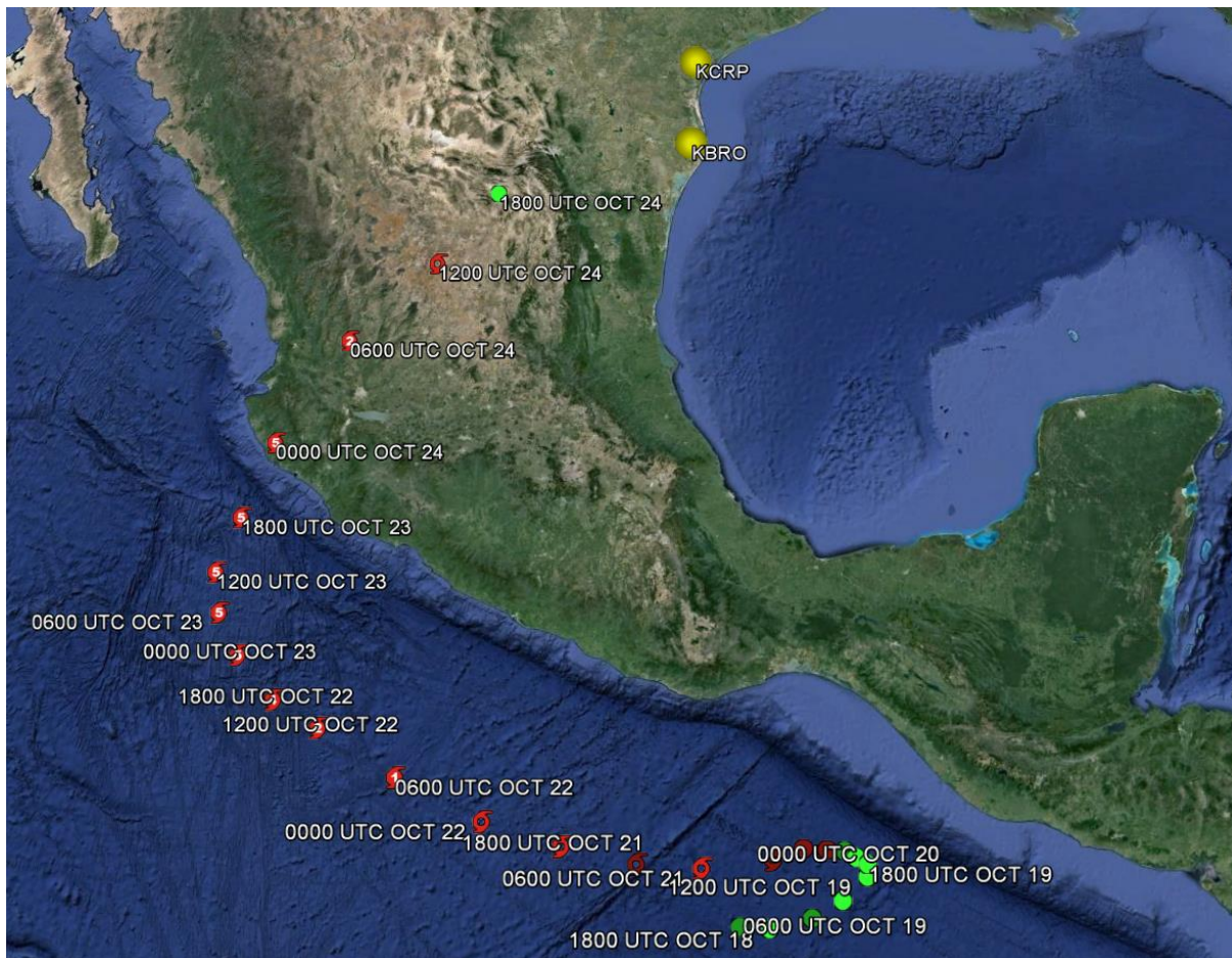
Figure 3. Hurricane Patricia best track and NWS sounding locations.
