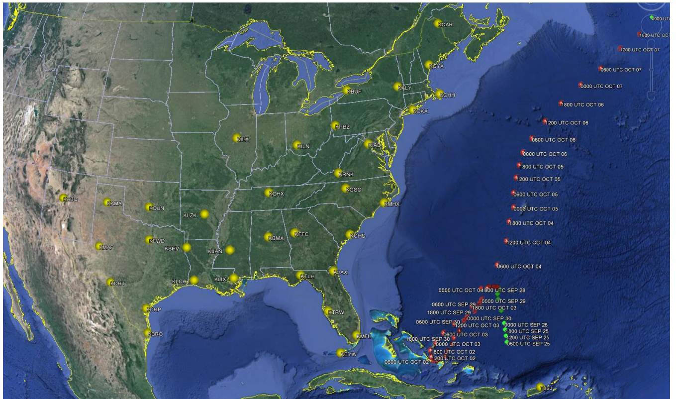
Figure 2. Hurricane Joaquin best track and NWS sounding locations.
