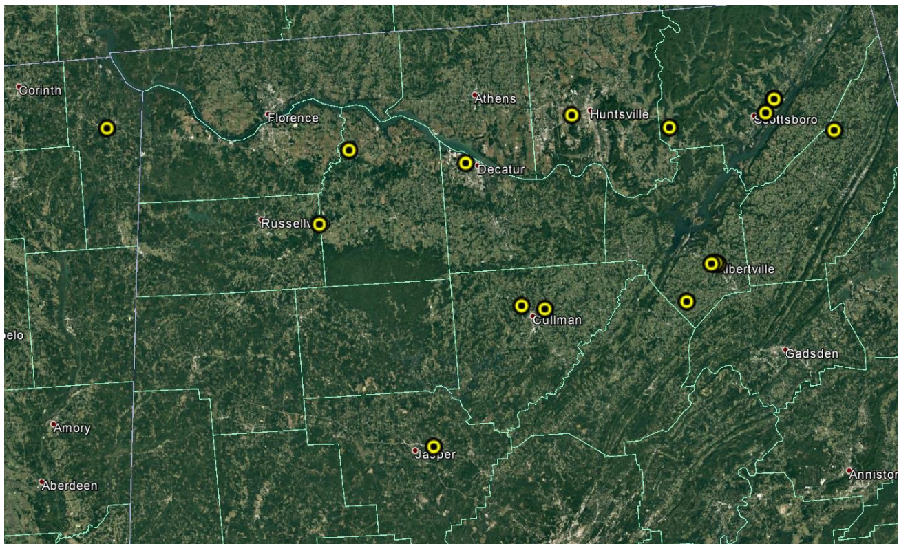
Figure 1. Location of VORTEX-SE_2017 NOAA/ARL/ATDD mobile radiosonde sites.
