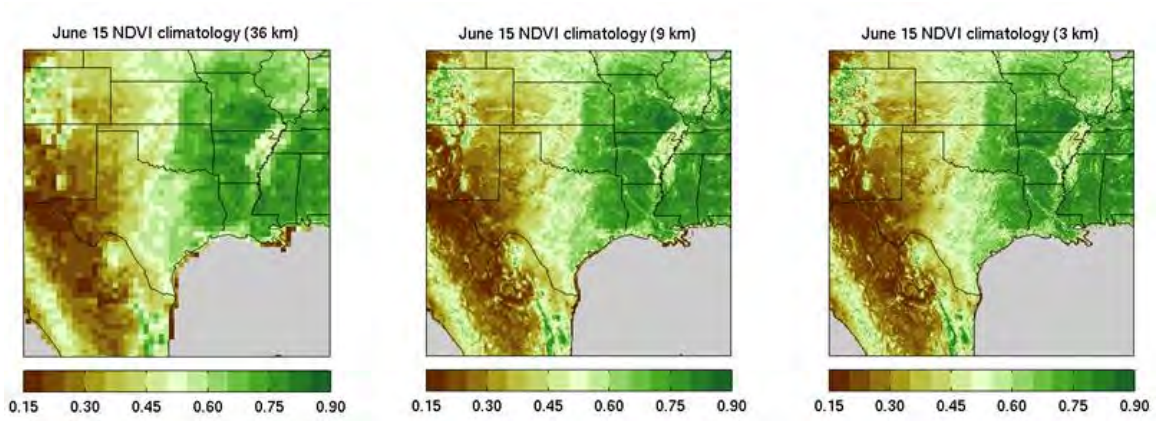
Figure 3: Example of ancillary NDVI climatology data displayed on the SMAP 36-km, 9-km, and 3-km grids.
