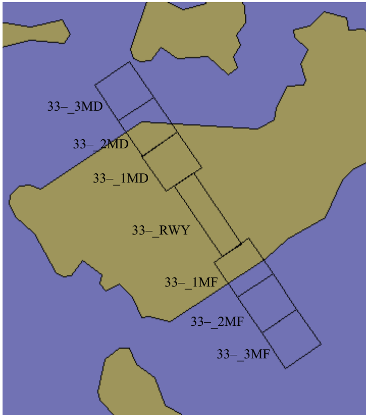
Figure 119 Configuring Protected Areas for TDWR
