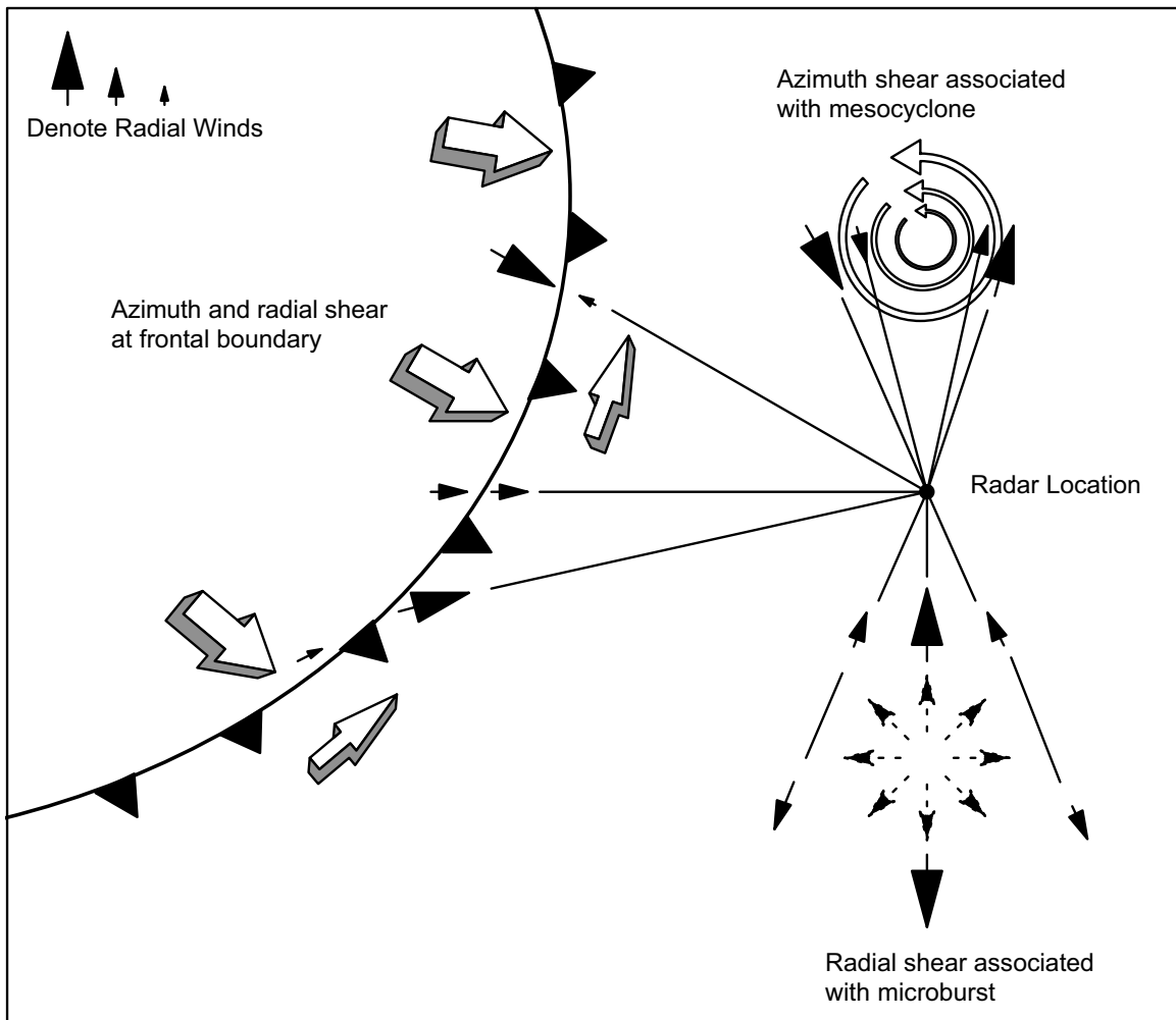
Figure 62 Schematic Examples of Wind Shear
