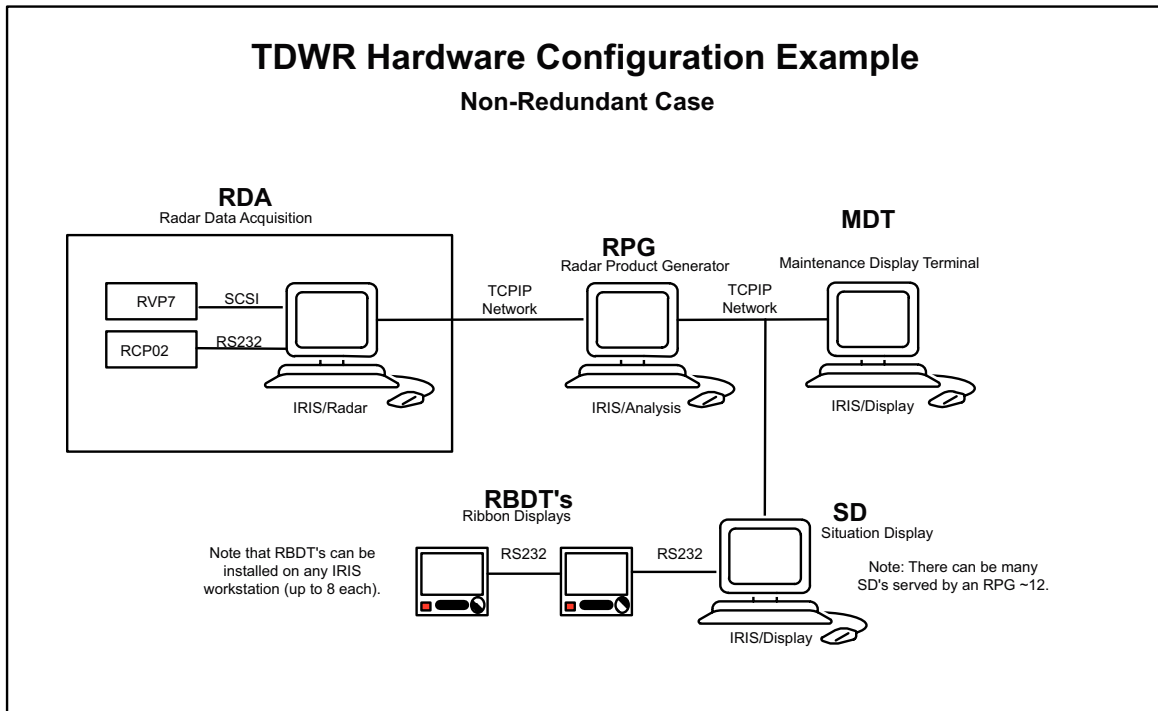
Figure 117 IRIS/TDWR Hardware Configuration Example
