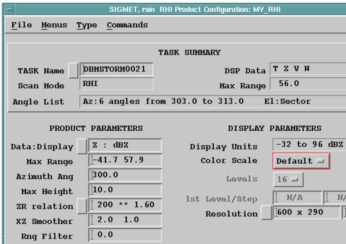
Figure 20 RHI Example Configuration
