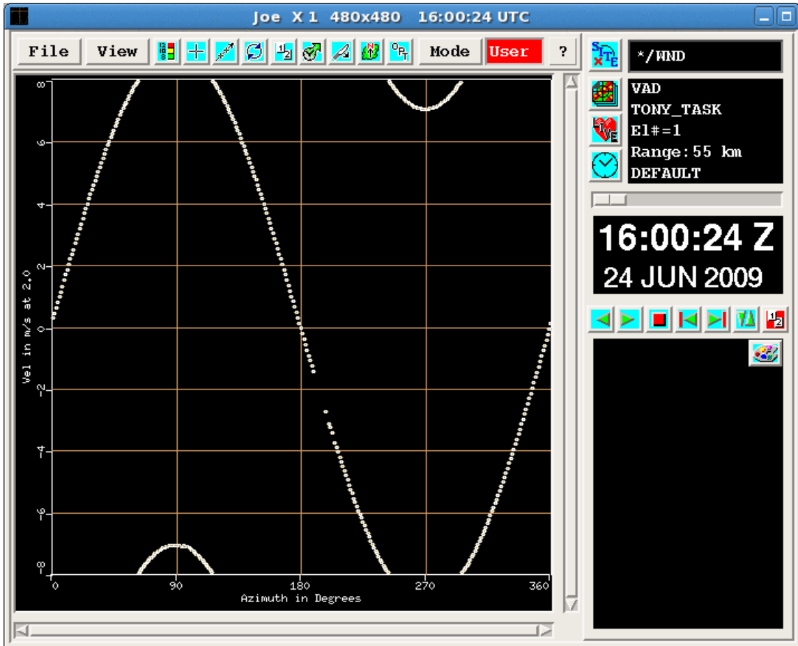
Figure 91 Example of Velocity Azimuth Display
