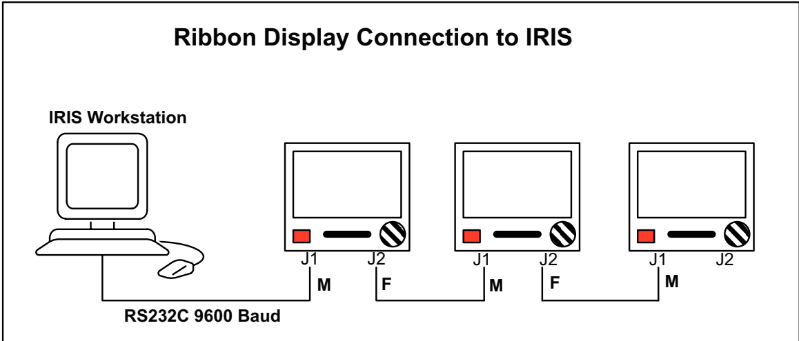
Figure 120 Dale Ribbon Display Installation
