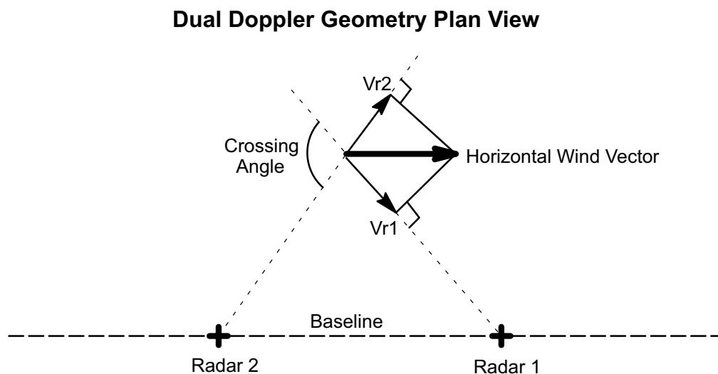
Figure 58 Dual Doppler Geometry Plan View
