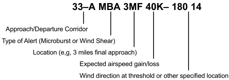
Figure 124 TDWR Ribbon Display Alert Messages
