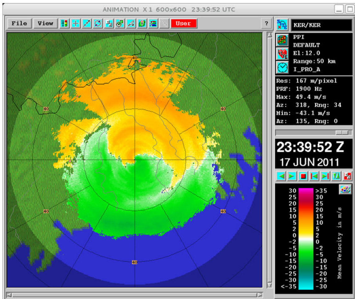
Figure 75 Example QLW: PPI Reflectivity (480 x 480 window size with range rings and overlay)
