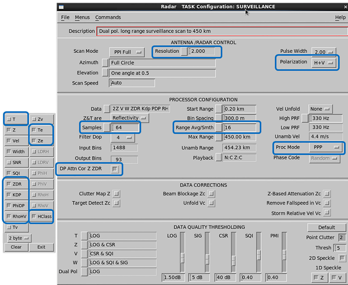
Figure 127 SURVEILLANCE Task Configuration -Dual Polarization
