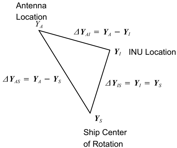
Figure 104 Vectors used for Velocity Correction In Earth Coordinates
