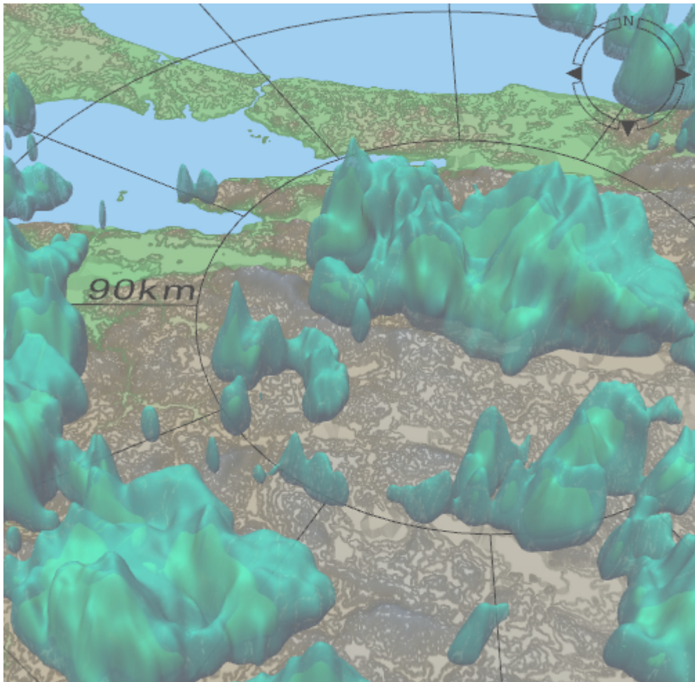
Figure 108 Example of Surface Rendering
