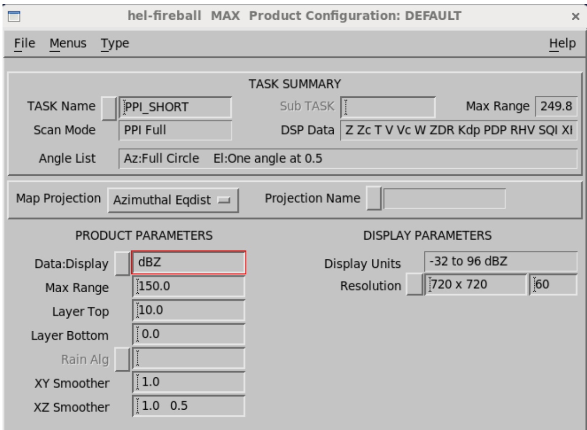
Figure 11 MAX Example Configuration
