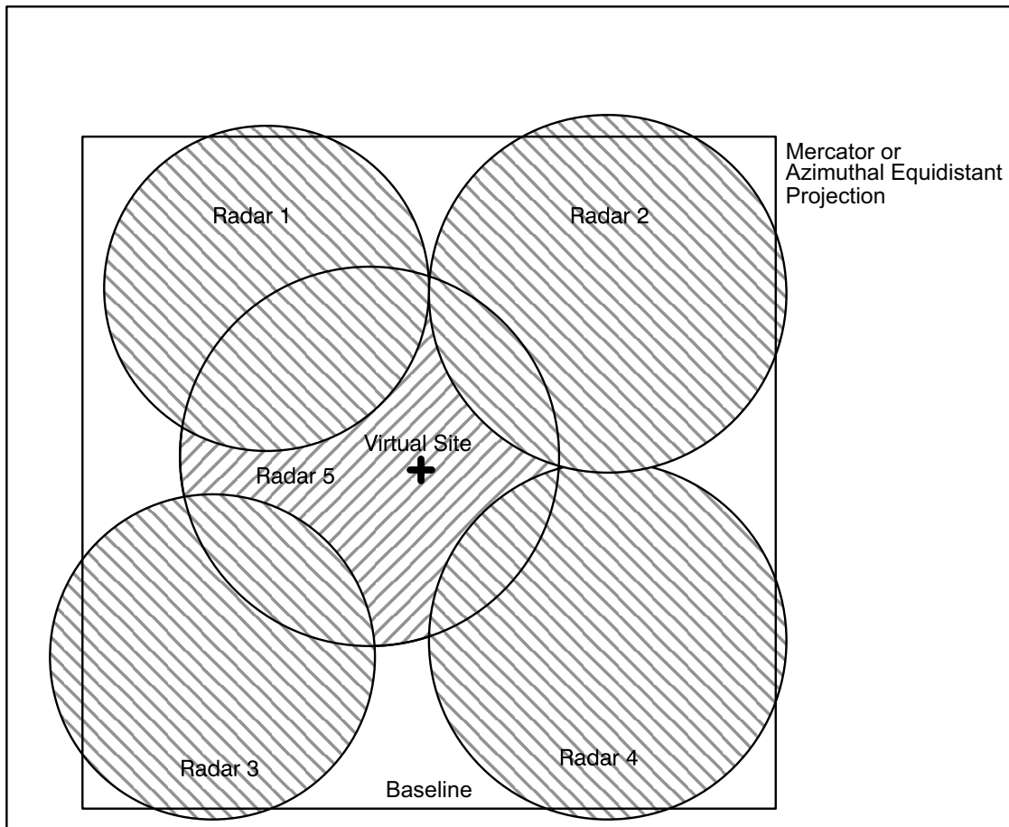
Figure 45 Example of Composite Projection Geometry
