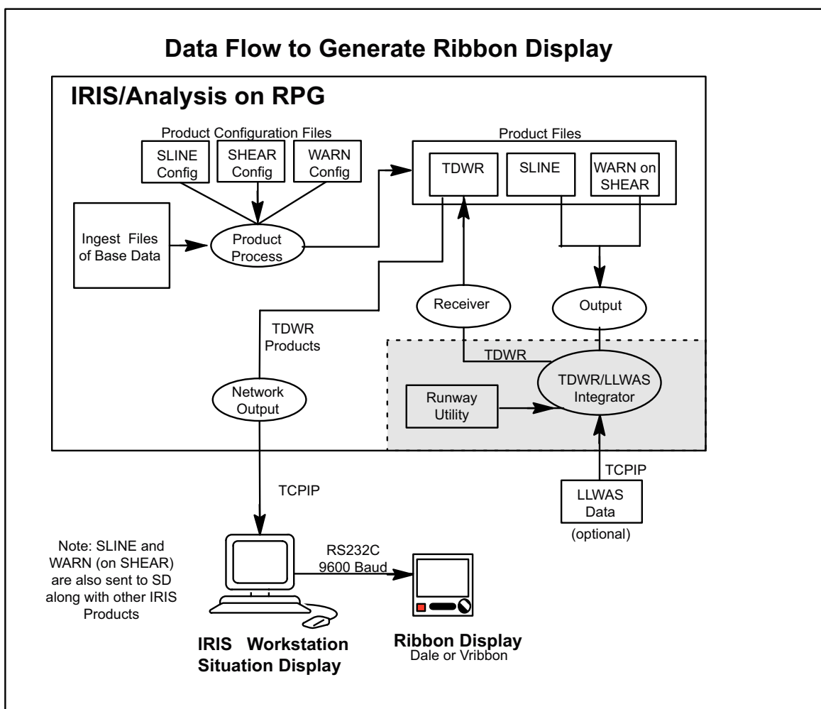
Figure 118 Data Flow for Generating TDWR Ribbon Display Products
