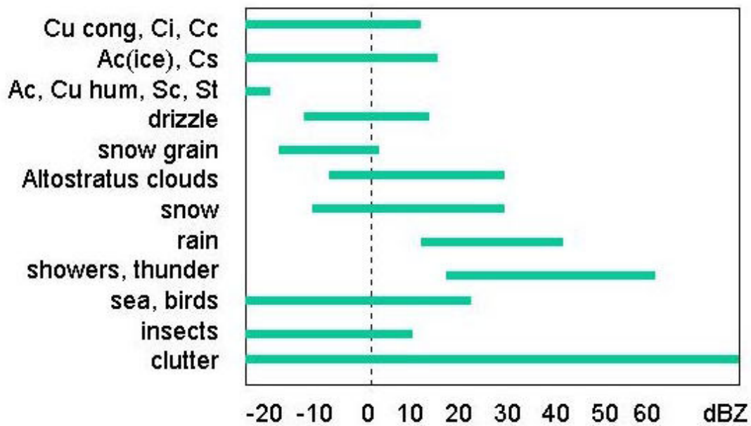
Figure 101 dBZ Values for Various Phenomena
