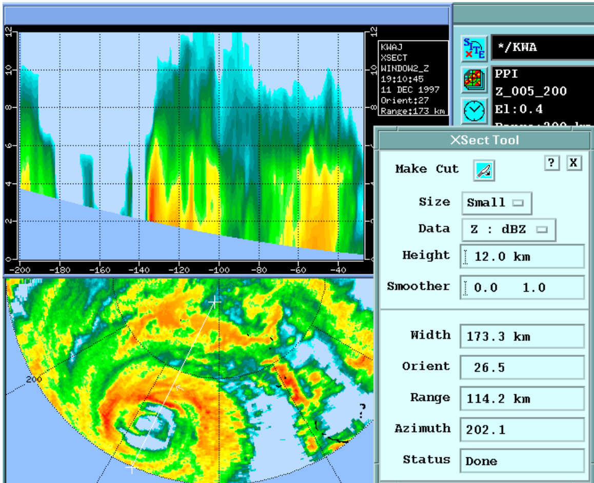
Figure 88 Cross-section with Typhoon Example
