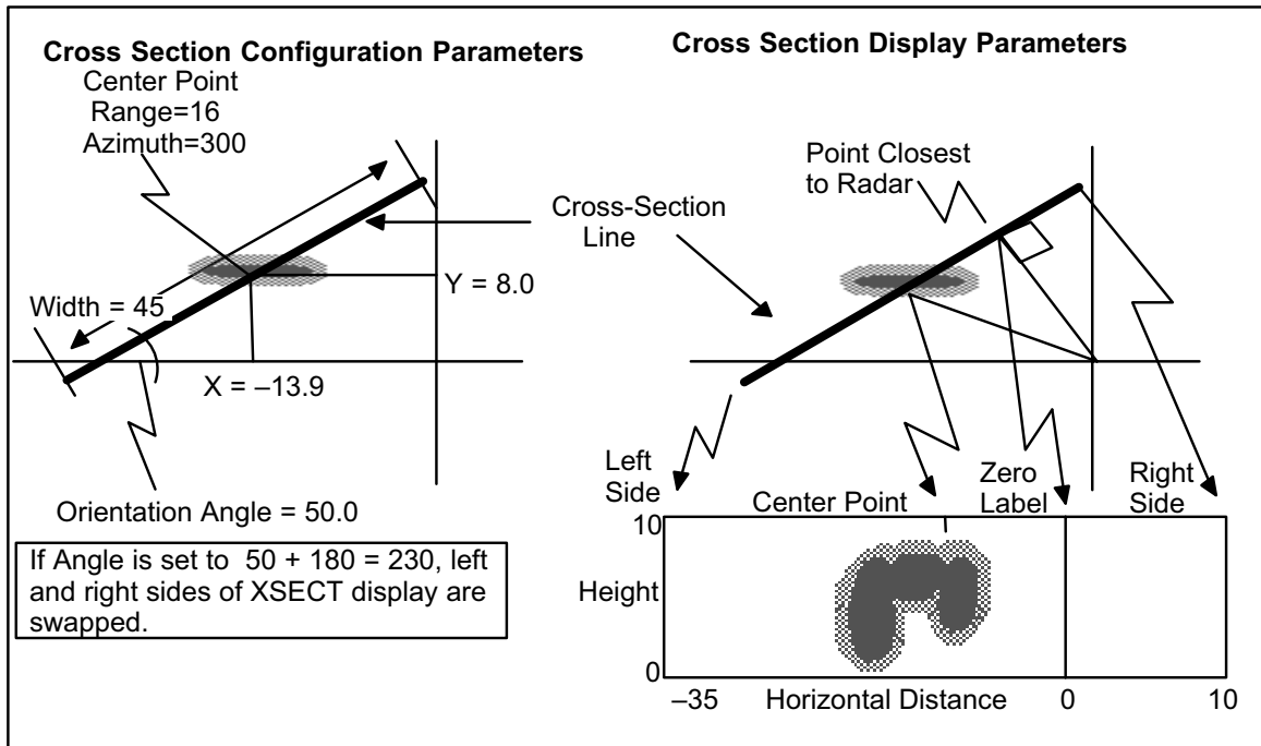
Figure 41 Cross Section Geometry
