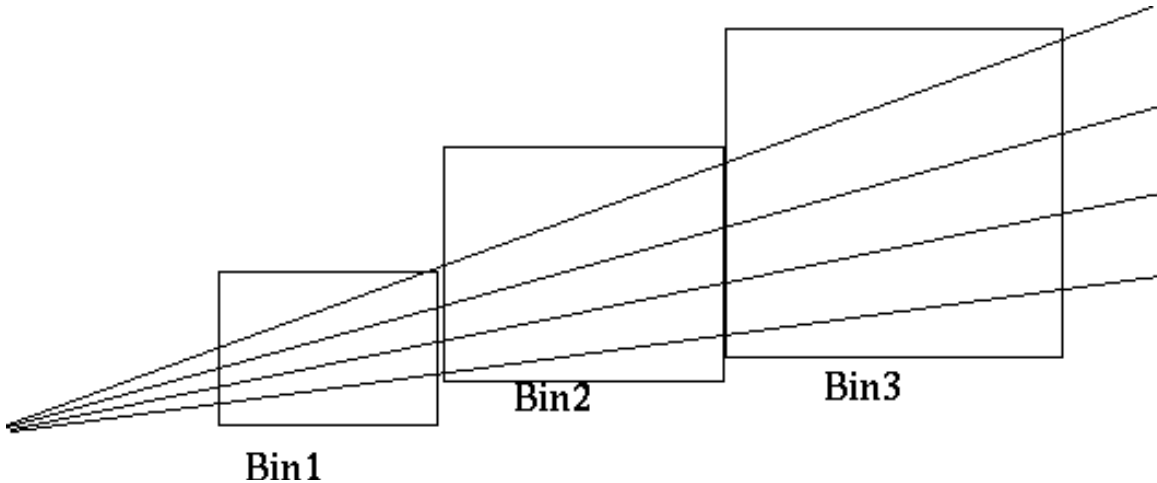
Figure 100 Range Bin Geometry
