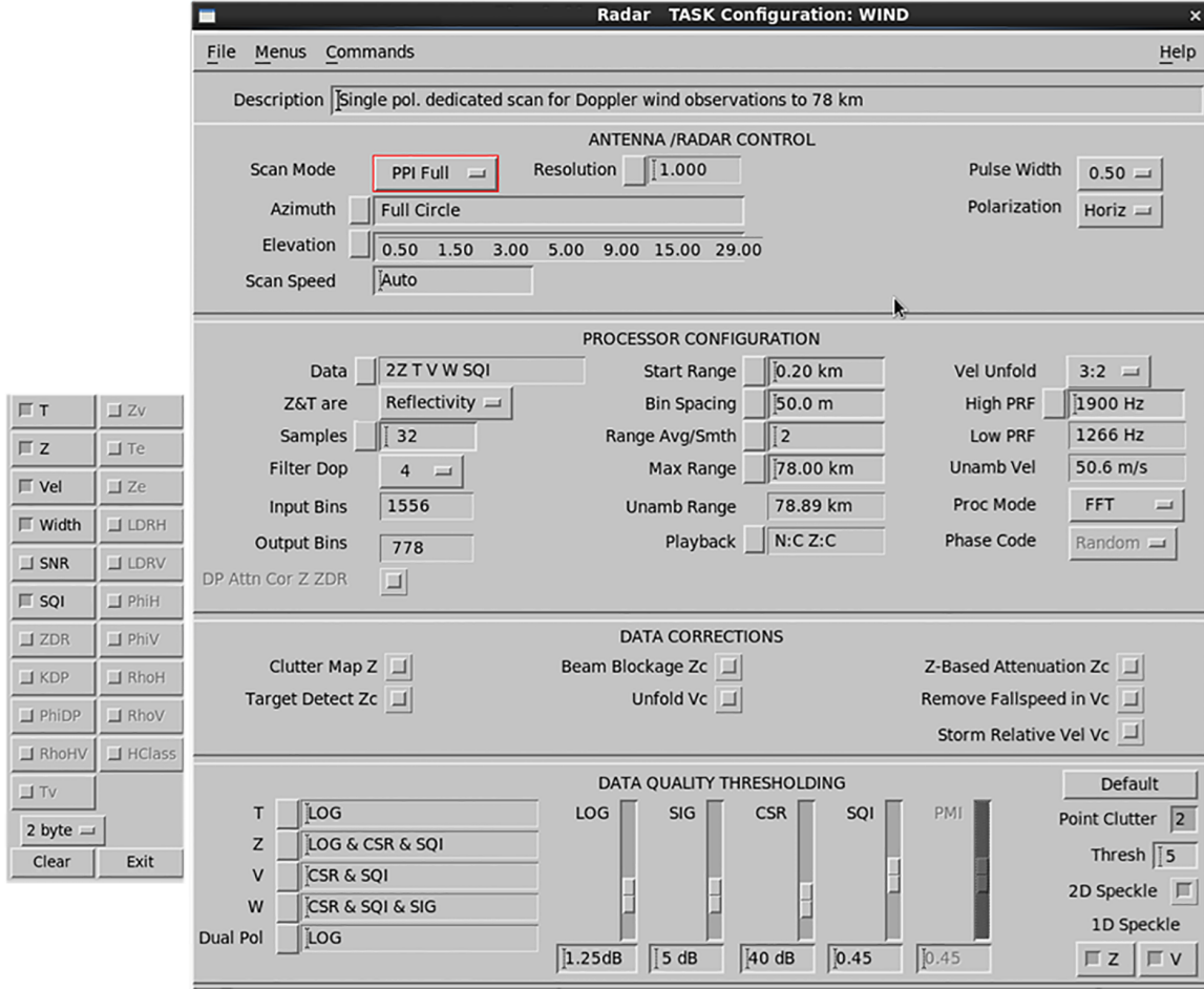
Figure 130 WIND Task Configuration
