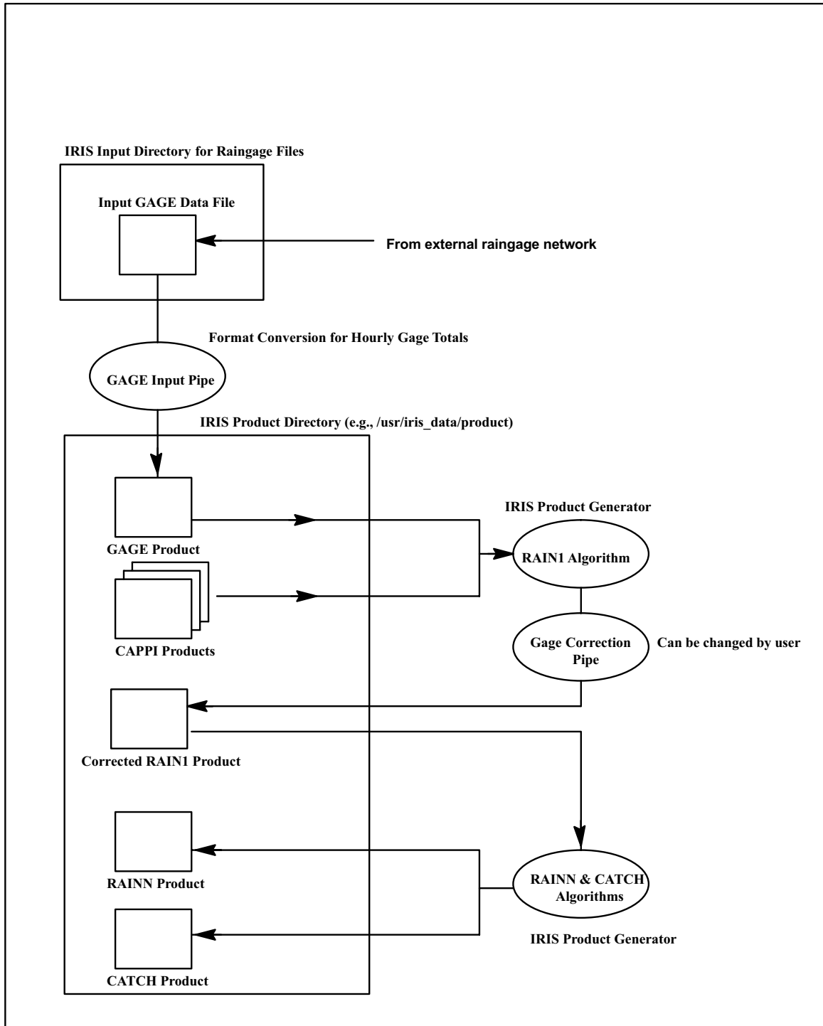
Figure 126 RAIN1 Raingage Correction Data Flow
