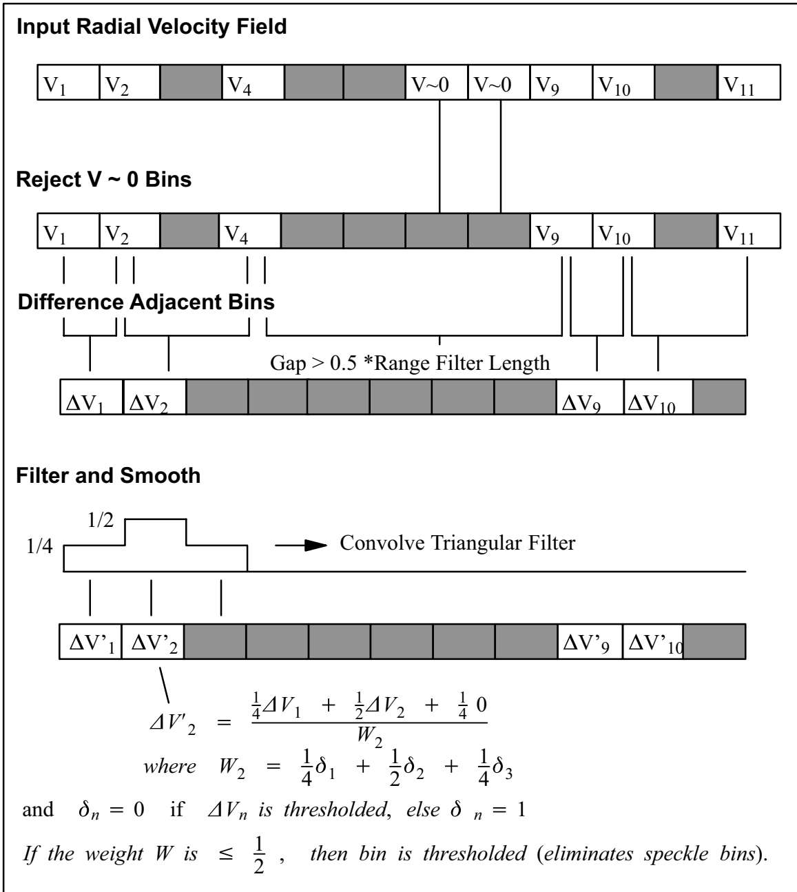
Figure 63 Radial Shear Algorithm Schematic
