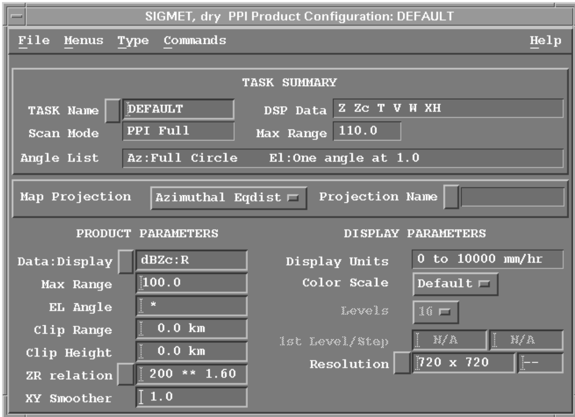
Figure 16 PPI Example Configuration
