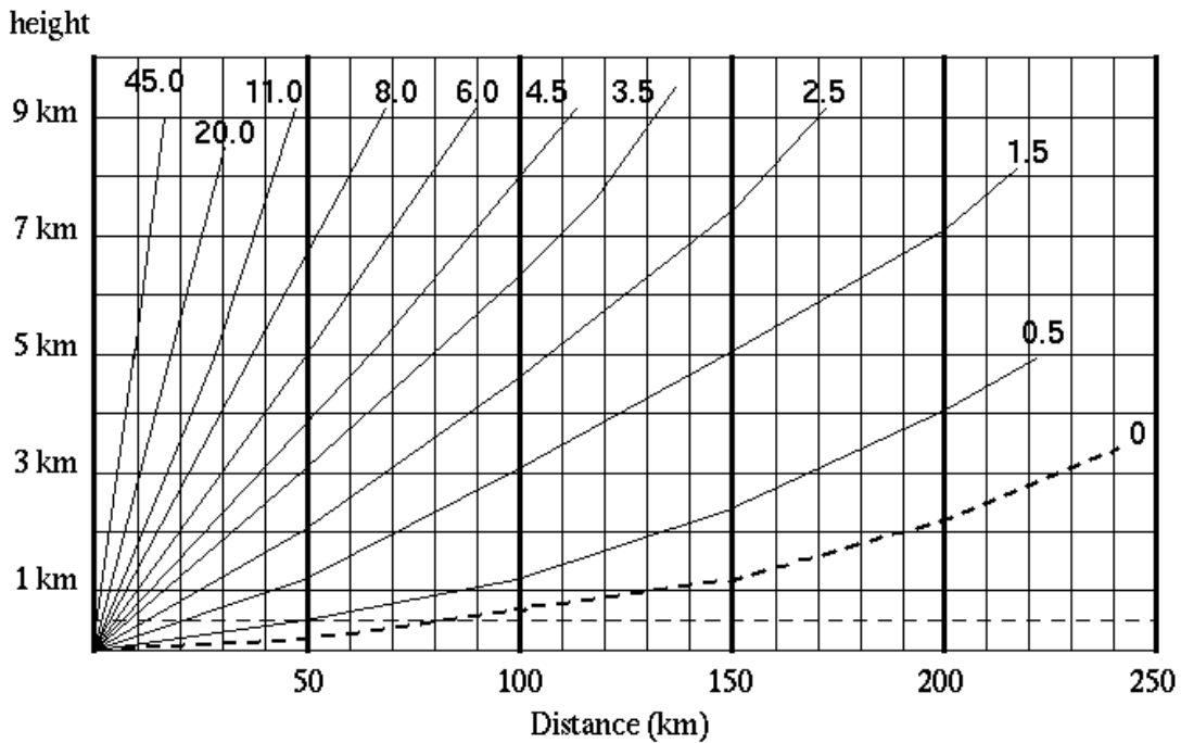
Figure 102 Beam Height vs. Range
