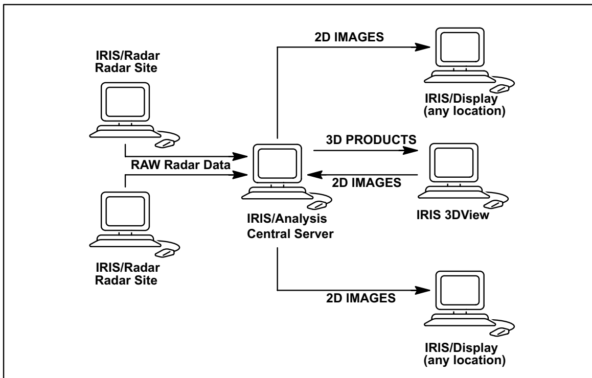
Figure 106 IRIS 3DView Data Flow
