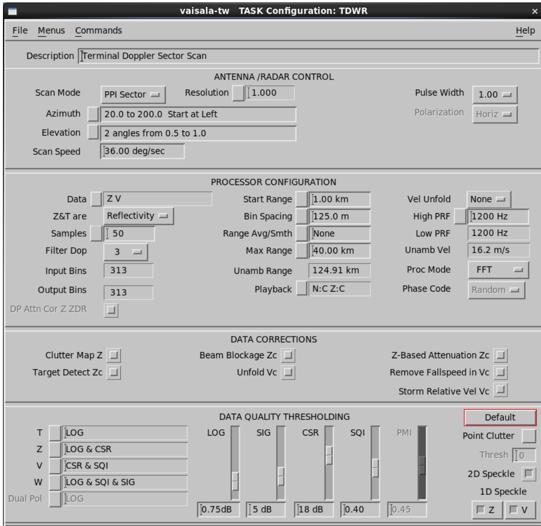
Figure 65 TASK Configuration for Microburst Detection
