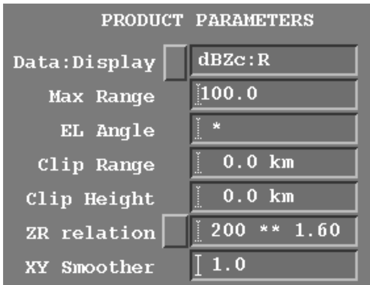
Figure 16 PPI Example Configuration
