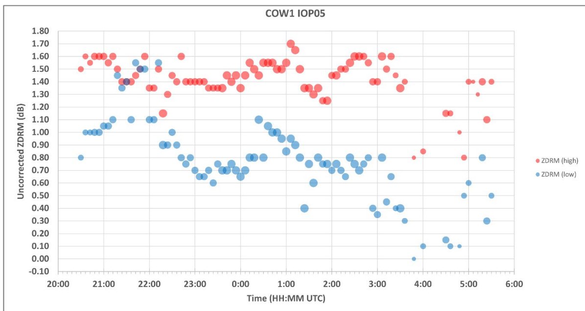
Figure 4: Measured COW1 ZDRM offsets from VER scans during IOP05 on 22-23 February 2022. Red bubbles represent the high frequency channel and blue bubbles represent the low frequency channel. The size of the bubbles represents the confidence in the offset value, where larger bubbles denote larger confidence.
