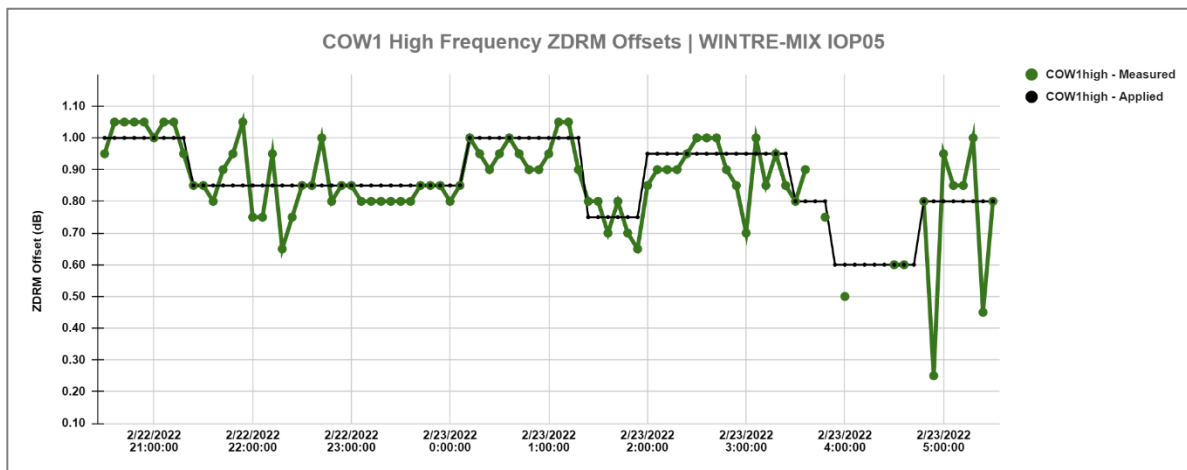
Figure 5: Measured (green) and applied (black) ZDRM offsets for COW1 IOP05.
