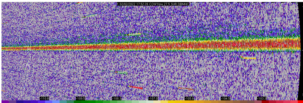
Figure 2: A solar spike observed in the horizontal power field (DBMHC) by the COW1 radar on 2 February 2022.
