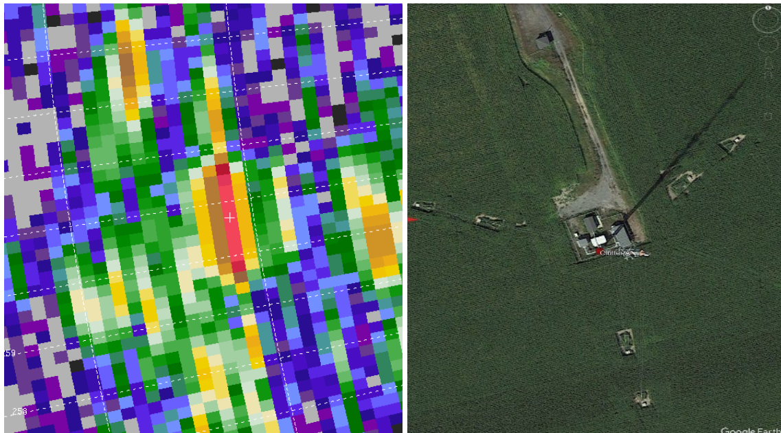
Figure 3: (Left) Radar reflectivity (DBZHC) of a cell tower clutter target (Right) observed by the COW1 radar 1.0° elevation SUR scan on 3 February 2022.
