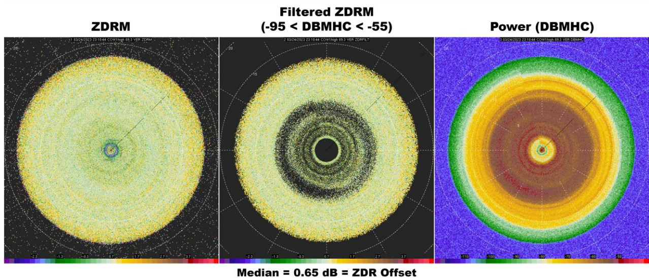
Figure 5: An example of a VER scan used to compute ZDR offsets. (Left) Un-filtered measured ZDR (ZDRM) from COW1 during IOP03. (Center) ZDRM filtered to remove values where returned power (DBMHC) is below -95 dBm or above -55 dBm and beyond a specific range from the radar. (Right) Power field measured by COW1 during this VER scan. The computed ZDR offset for this specific VER scan is shown below the center panel.
