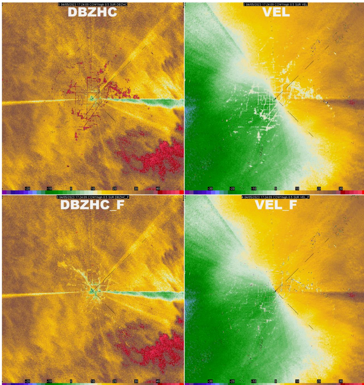
Figure 1: (Left) COW1 reflectivity product unfiltered (top) and clutter-filtered (bottom). (Right) COW1 Doppler velocity product unfiltered (top) and clutter-filtered (bottom).
