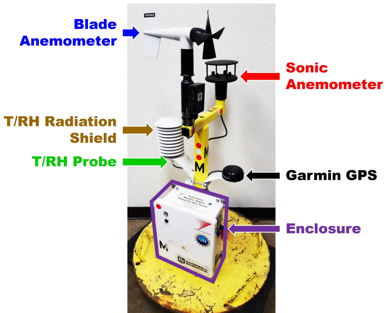
Figure 13: FARM quickly-deployable “pod” with weather instrumentation and components identified. A pressure sensor, battery, and datalogger is encompassed in the enclosure.
