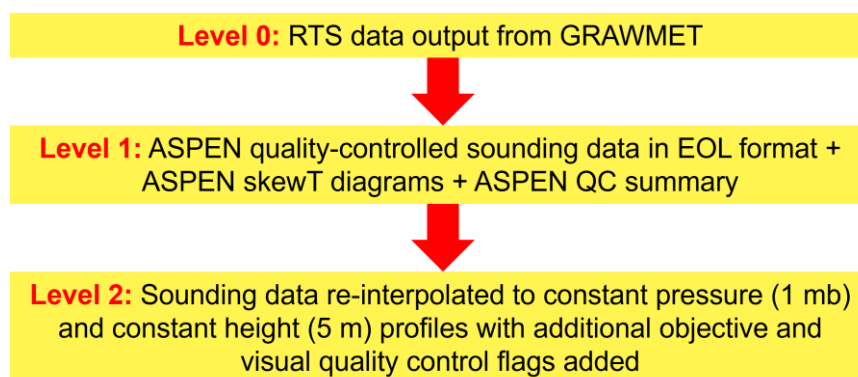
Figure 9: Sounding quality control flow diagram documenting the three main processing levels.
