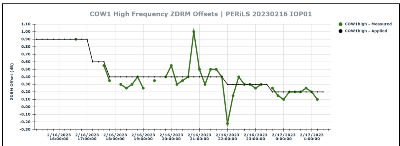
Figure 7: Measured (green) and applied (black) ZDRM offsets for COW1 high frequency channel data during IOP01 on 16 February 2023.
