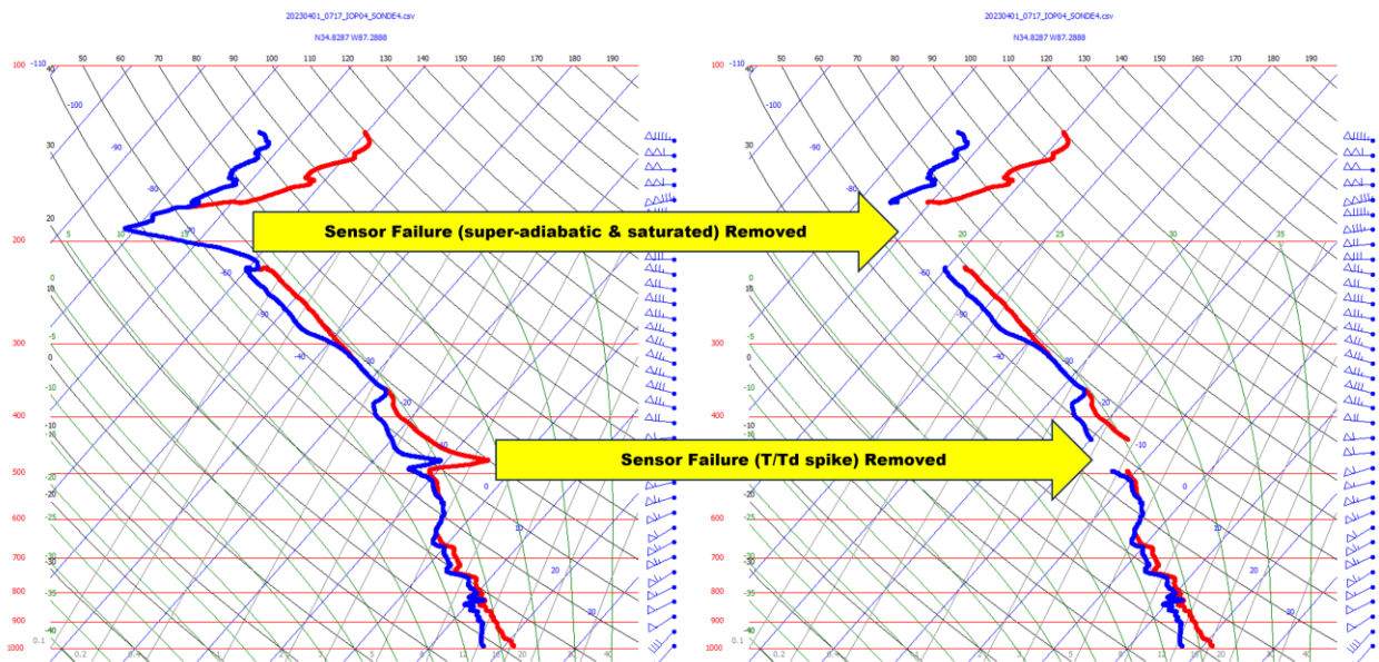
Figure 11: A skewT plot generated by ASPEN for a sounding that has two obvious layers of bad temperature and dewpoint data that corresponds with sensor failures. The left side shows the ASPEN processed sounding without ignoring the bad temperature and dewpoint values, and the right side shows after ignoring bad temperature and dewpoint values.
