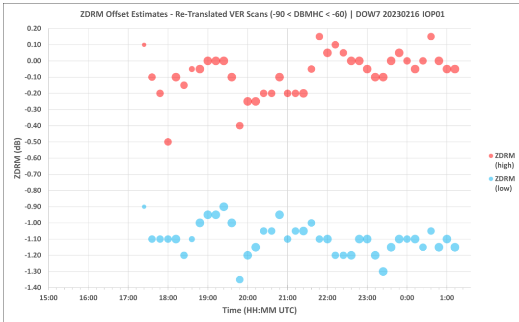
Figure 6: Measured DOW7 ZDRM offsets from VER scans during IOP01 on 16 February 2023. Red (blue) bubbles represent the high (low) frequency channel. The size of the bubbles represents the confidence in the offset value, where larger bubbles denote larger confidence.
