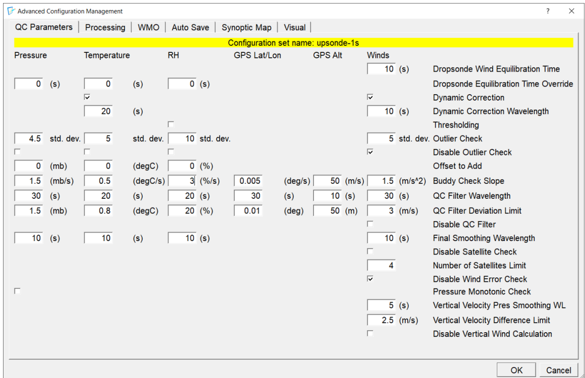
Figure 10: ASPEN quality control parameters for upsonde-1s data used to process the FARM PERiLS 2023 sounding dataset.
